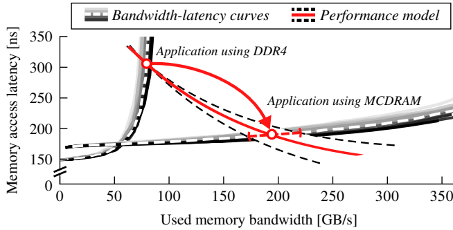
Fig. 8. Graphical interpretation of a performance estimation as a merged solution of Sections 3 and 4.4.
