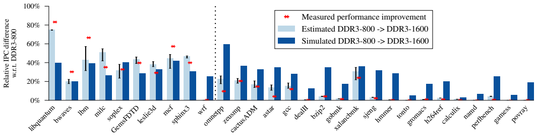
Fig. 14. Sandy Bridge, DDR3-800→1600: Comparison of the estimated (PROFET) and simulated (ZSim+DRAMSim2) performance improvement. Estimations of PROFET correspond to the real-system measurements much better than the simulated performance.
