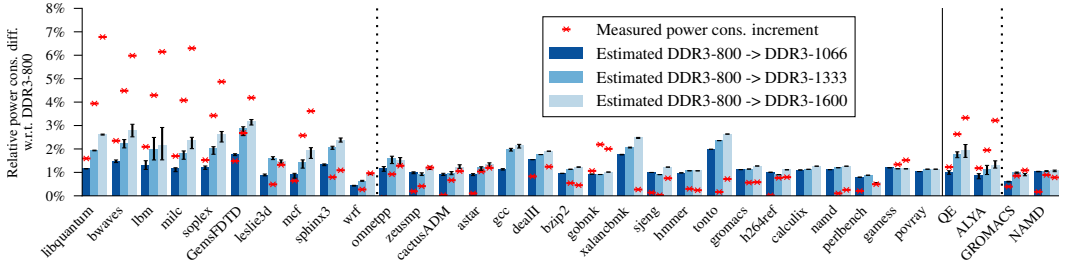
Fig. 12. Sandy Bridge, DDR3-800→1066/1333/1600: DRAM frequency has a minor impact on the overall server power consumption. Increasing DRAM frequency from DDR3-800 to DDR3-1600 (100% increment) causes average power increment of only 2%.
