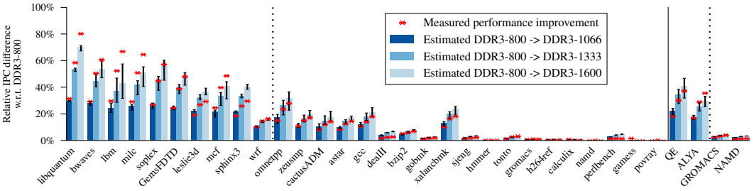
Fig. 10. Sandy Bridge, DDR3-800 → 1066/1333/1600: Changing the DRAM frequency has a significant performance impact. PROFET’s performance model estimations are precise, with low error bars, and accurate, with small difference from the values measured on the actual hardware.
