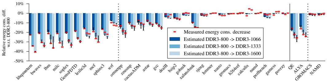
Fig. 13. Sandy Bridge, DDR3-800→1066/1333/1600: DRAM frequency has a significant impact on the system energy consumption. Energy predictions of PROFET are precise, with low error bars, and accurate, with small difference from the actual values measured on real hardware.
